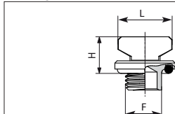
9/S - Plug with control bar and o-ring
