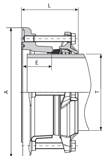
O.D. 160 and O.D. 200 to 315
