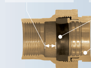
Section of a SE14 fitting
