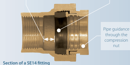
Section of a SE14 fitting
