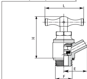
9/A - Drain tap with spout and o-ring
