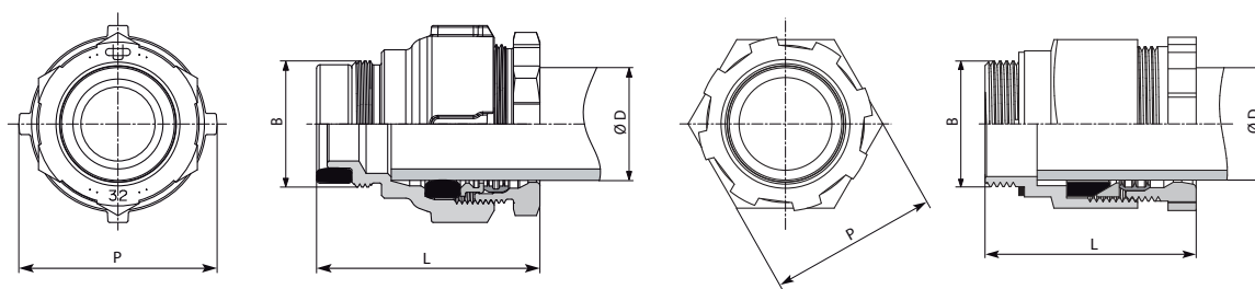
Self-sealing, with large gasket
